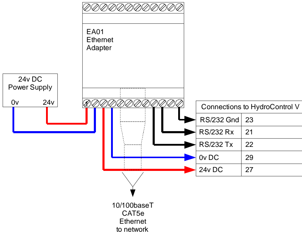
Figure 5: Connecting the Ethernet Adapter to Hydro-Control V
