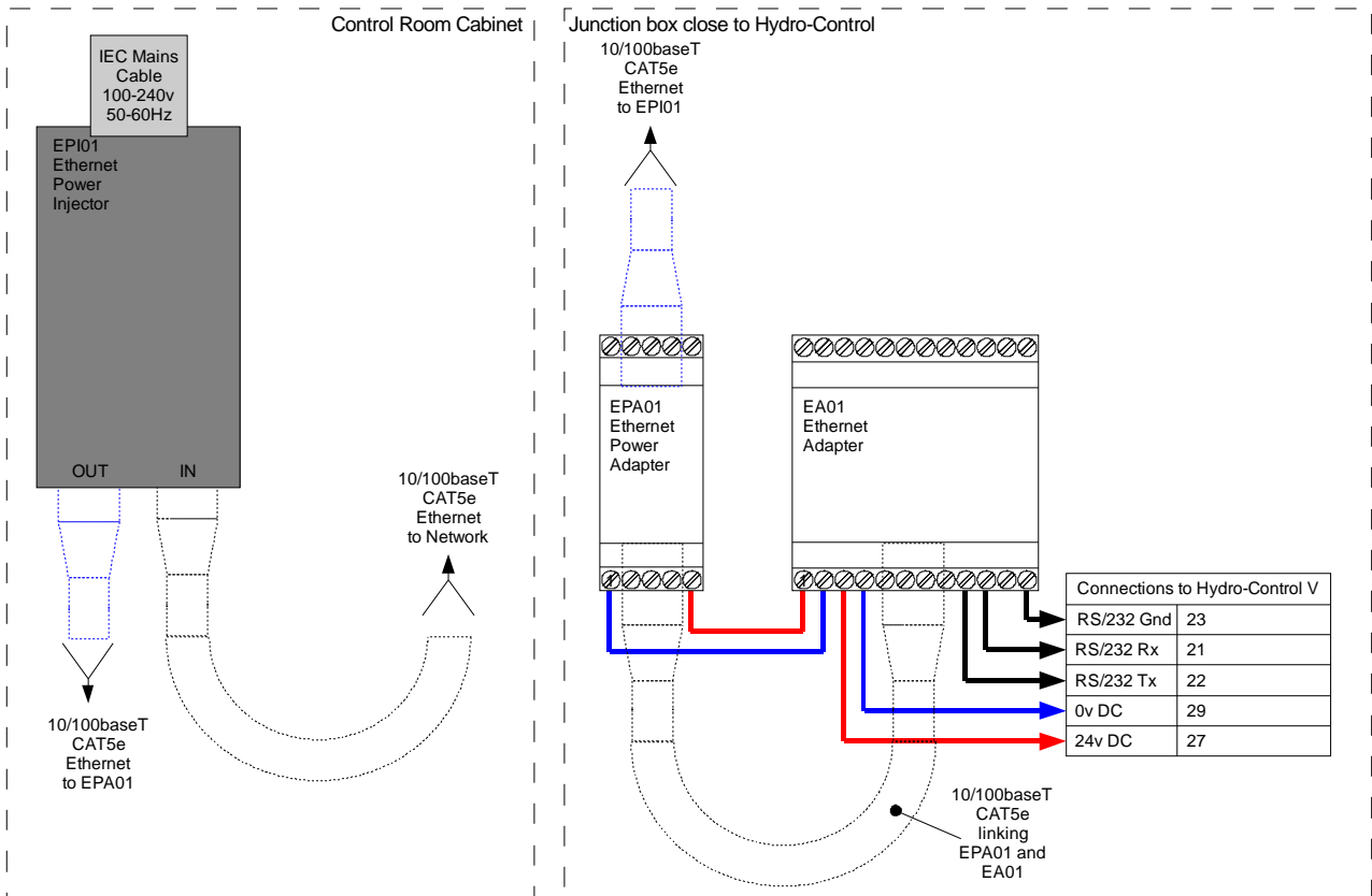
Figure 6: Connecting the Ethernet Adapter to Hydro-Control V with Power Over Ethernet Option Location of the Power Adapter (EPA01)
