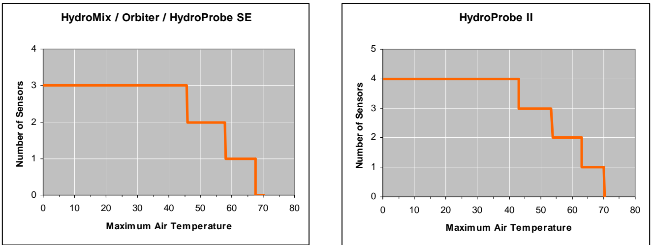
Figure 4: Maximum number of sensor connections
