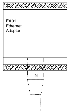
Figure 6: EA01 Terminal Identification
