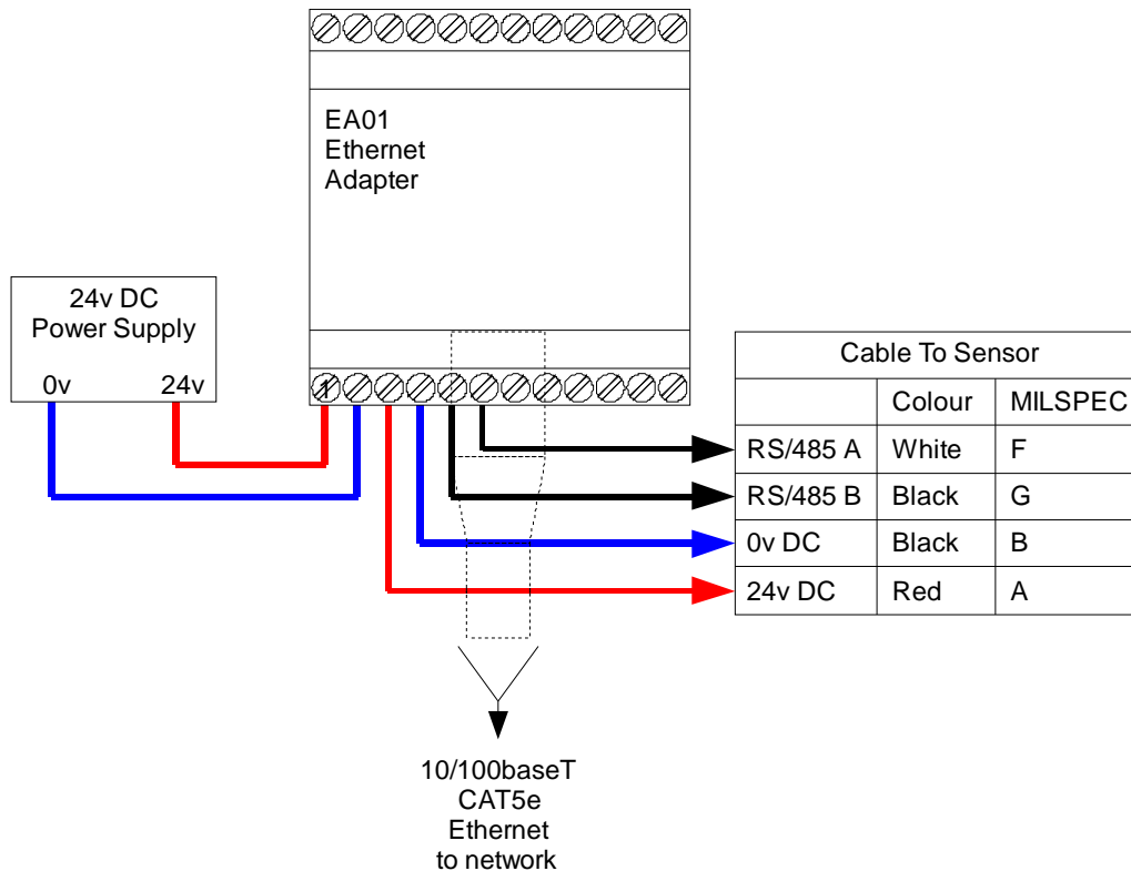
Figure 2: Connections for Ethernet Adapter only
